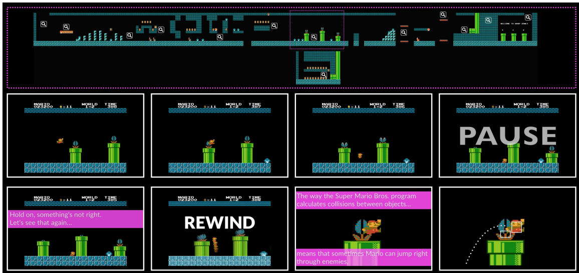
Figure 4. Key frames from a SMBI Game Inspector video illustrating collision detection and hitboxes
